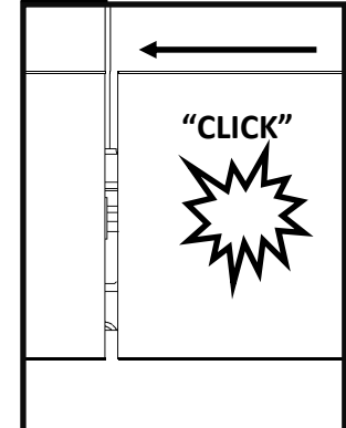
Push luminaires and together listen for a click as the joiner bracket is located.
